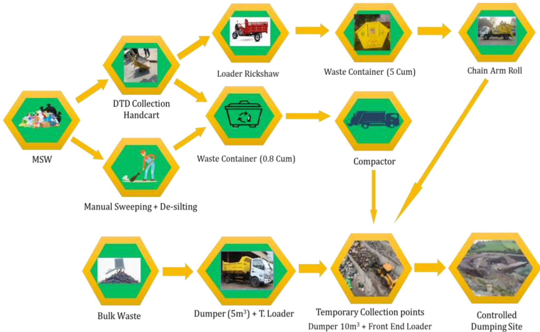
Figure 2. Proposed Operations Model of Urban Area
